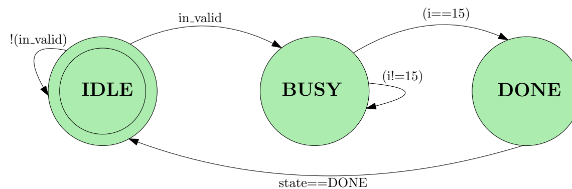
Control FSM
